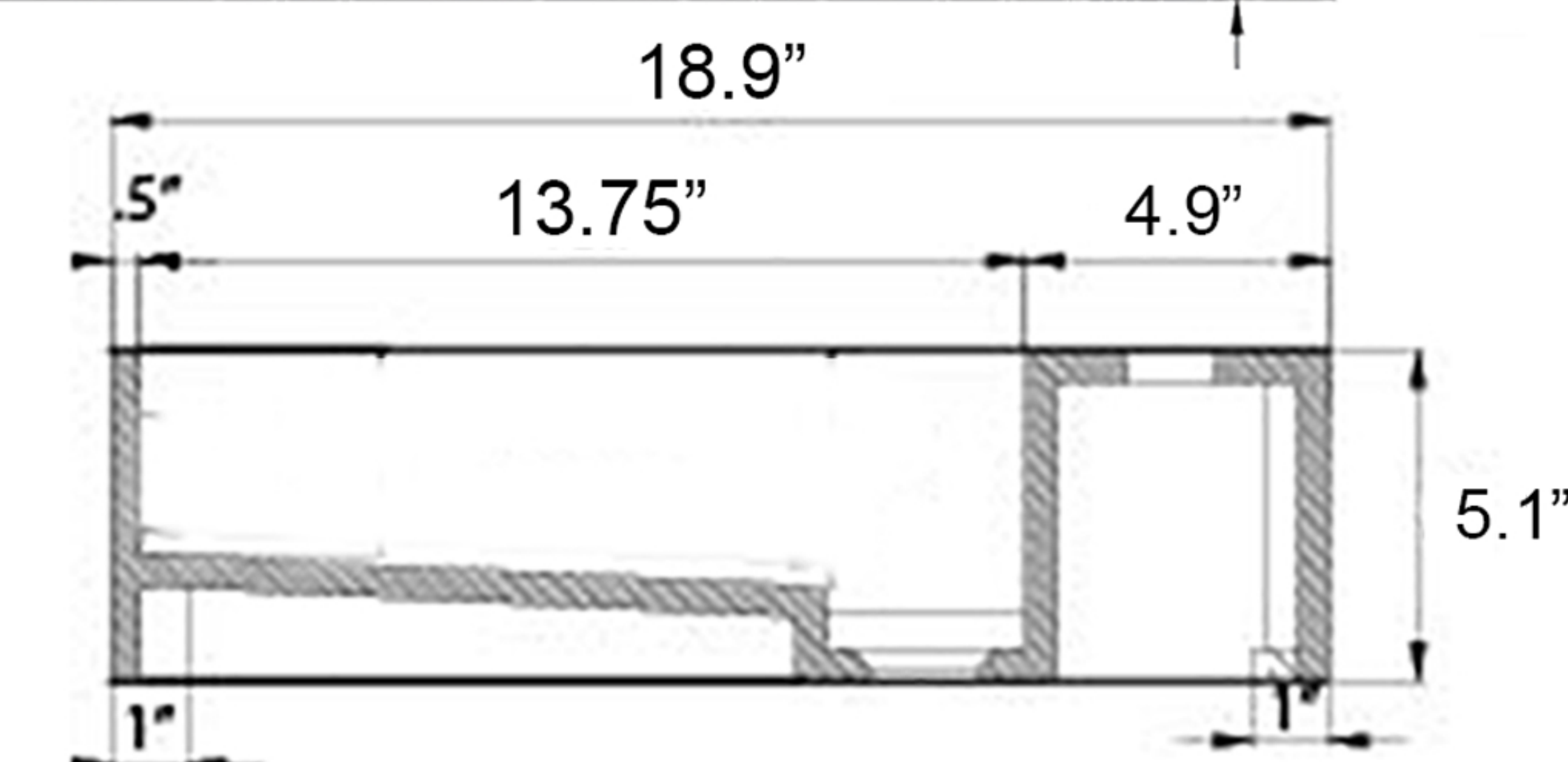
Side View
