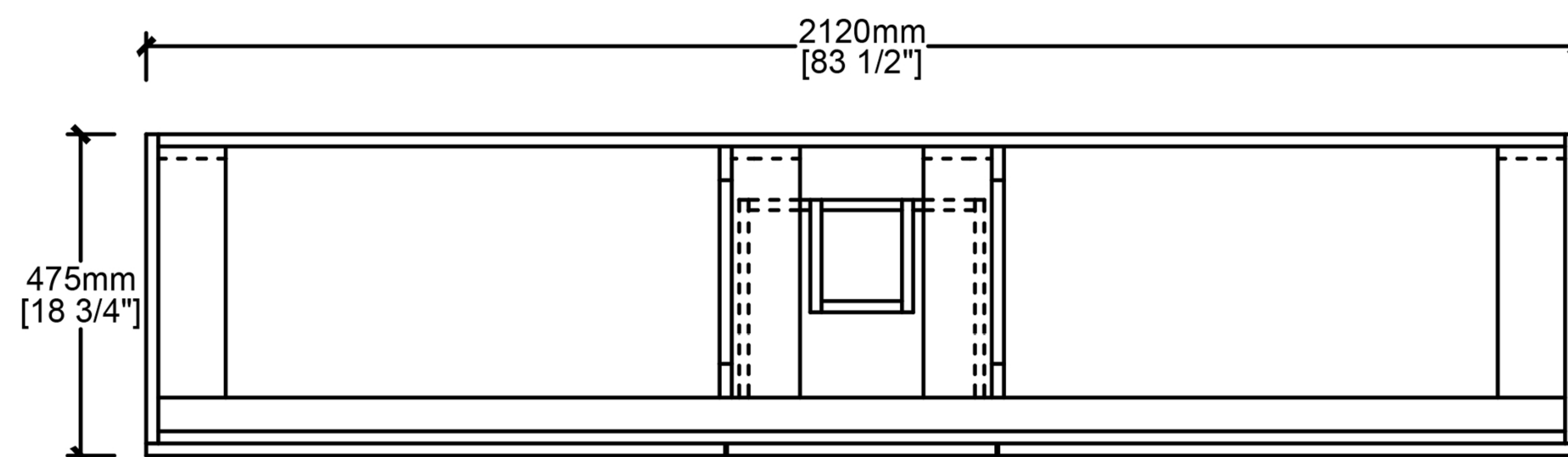
Top View
