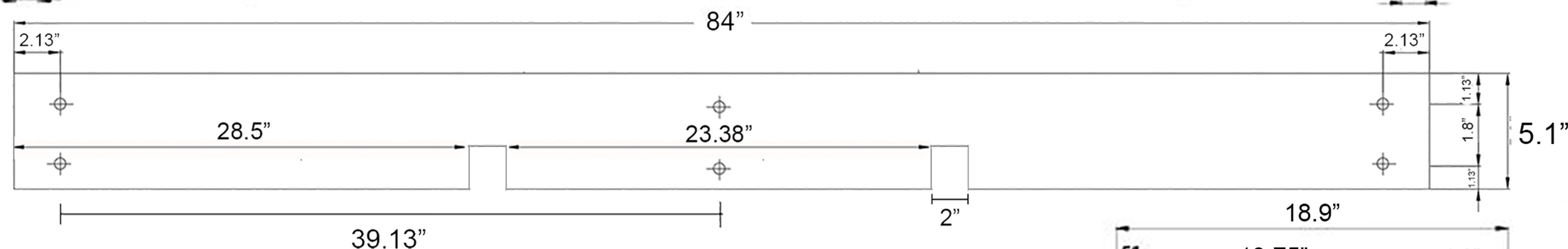
Rear View
