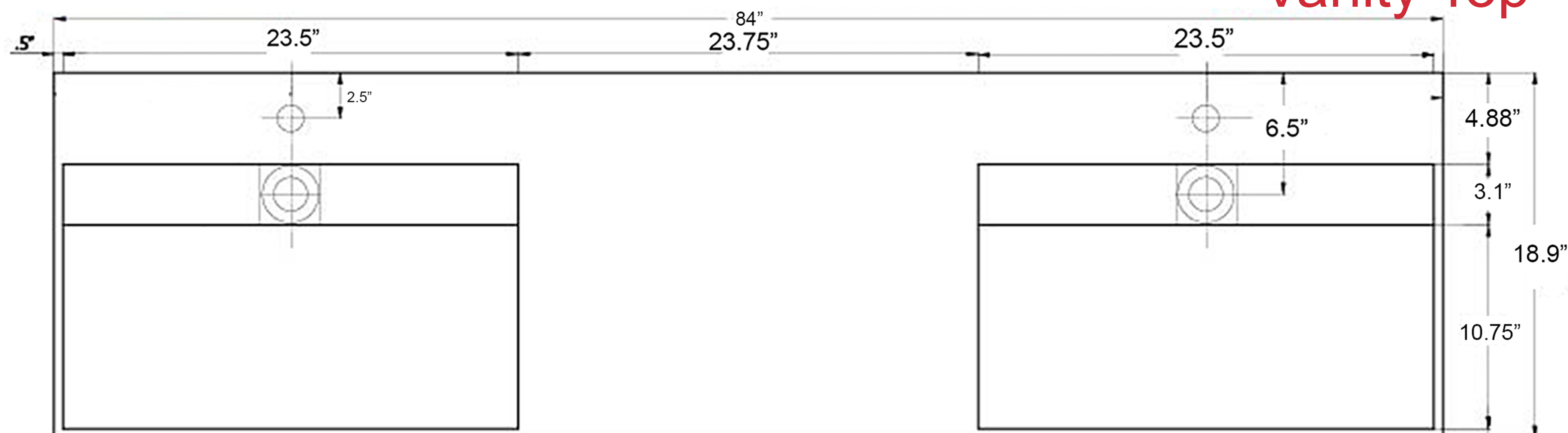
Top View
