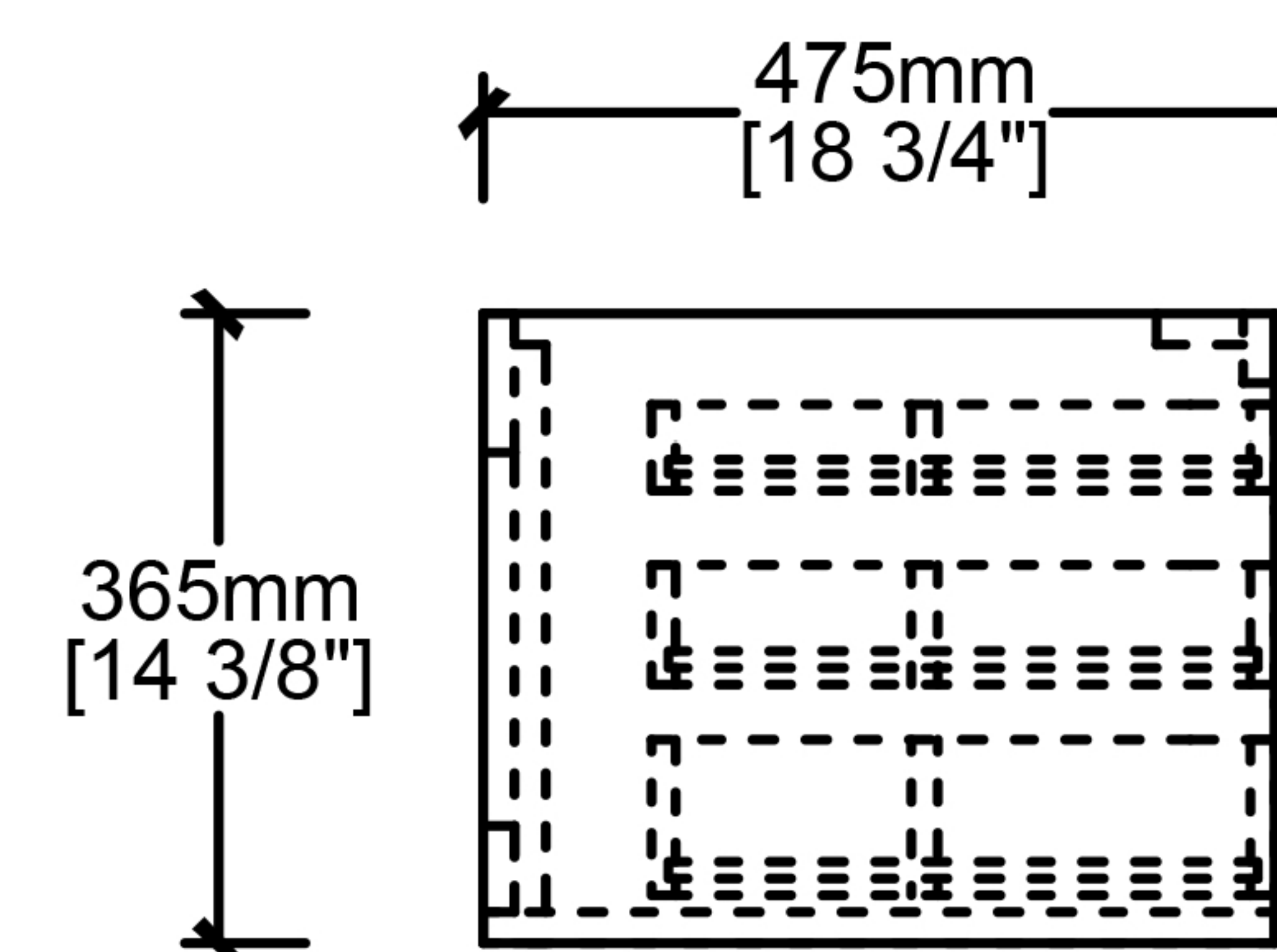
Side View
