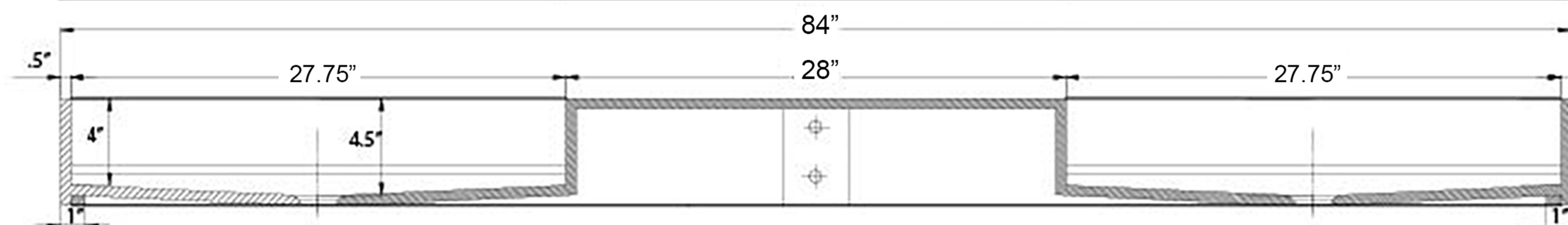
Front view
