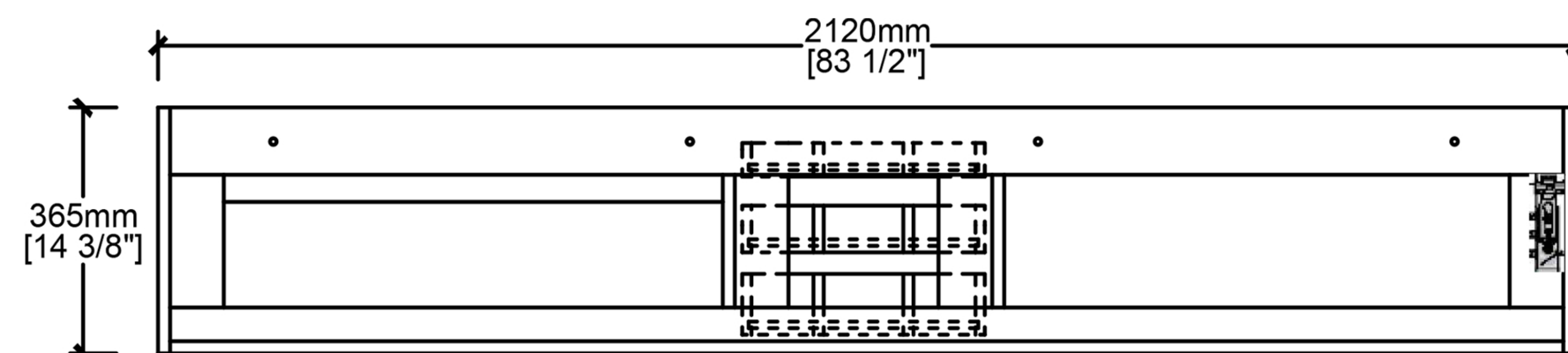
Rear view
