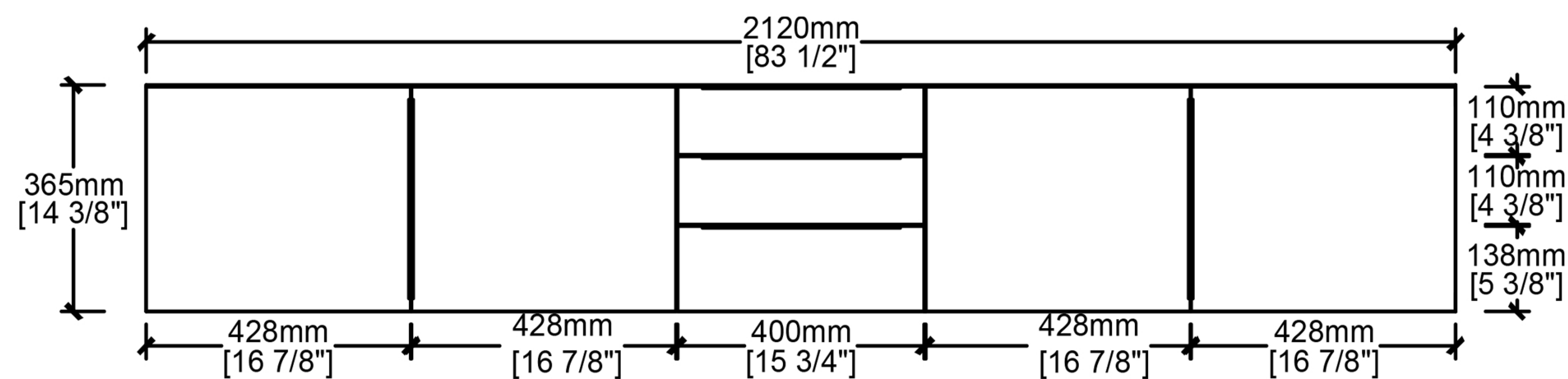
Front view
